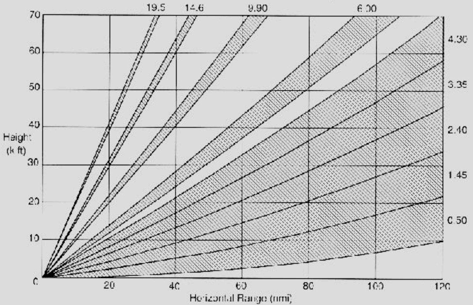
Figure 5.2 Alternative Scan Volume Coverage Pattern 21
